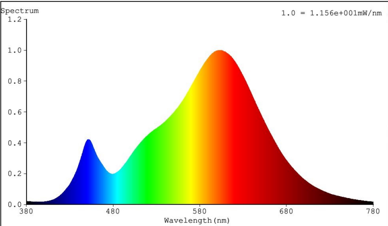
Spectral Distribution
