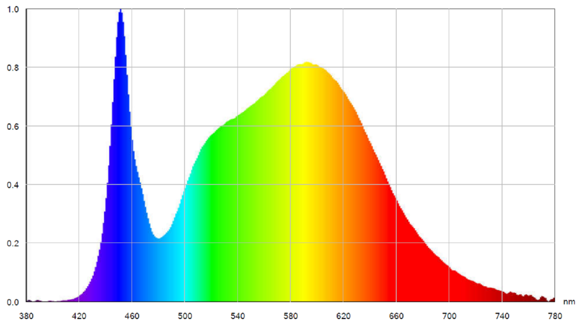
Spectrum Curve
