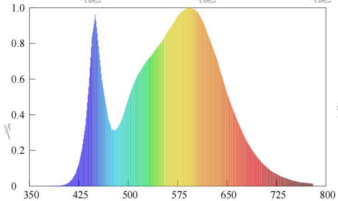
Spectral power distribution(4000k)
