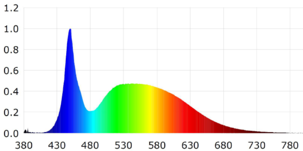
Spectral power distribution at 6500K
