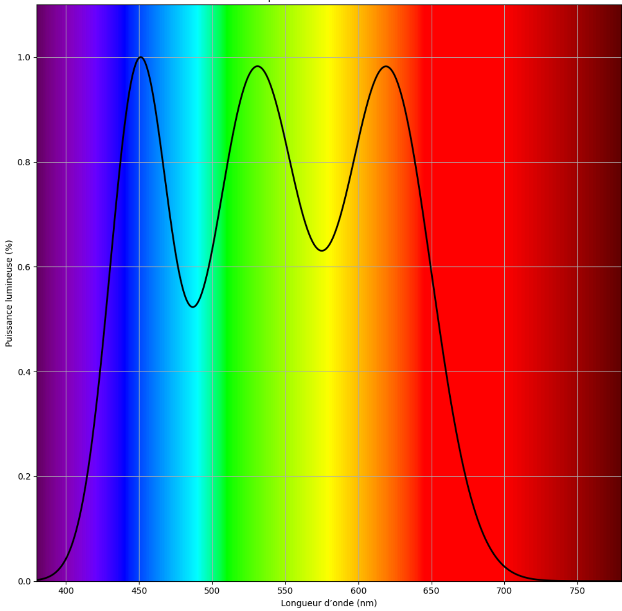
Distribution spectrale - Ruban LED RGB 72W Ra80
