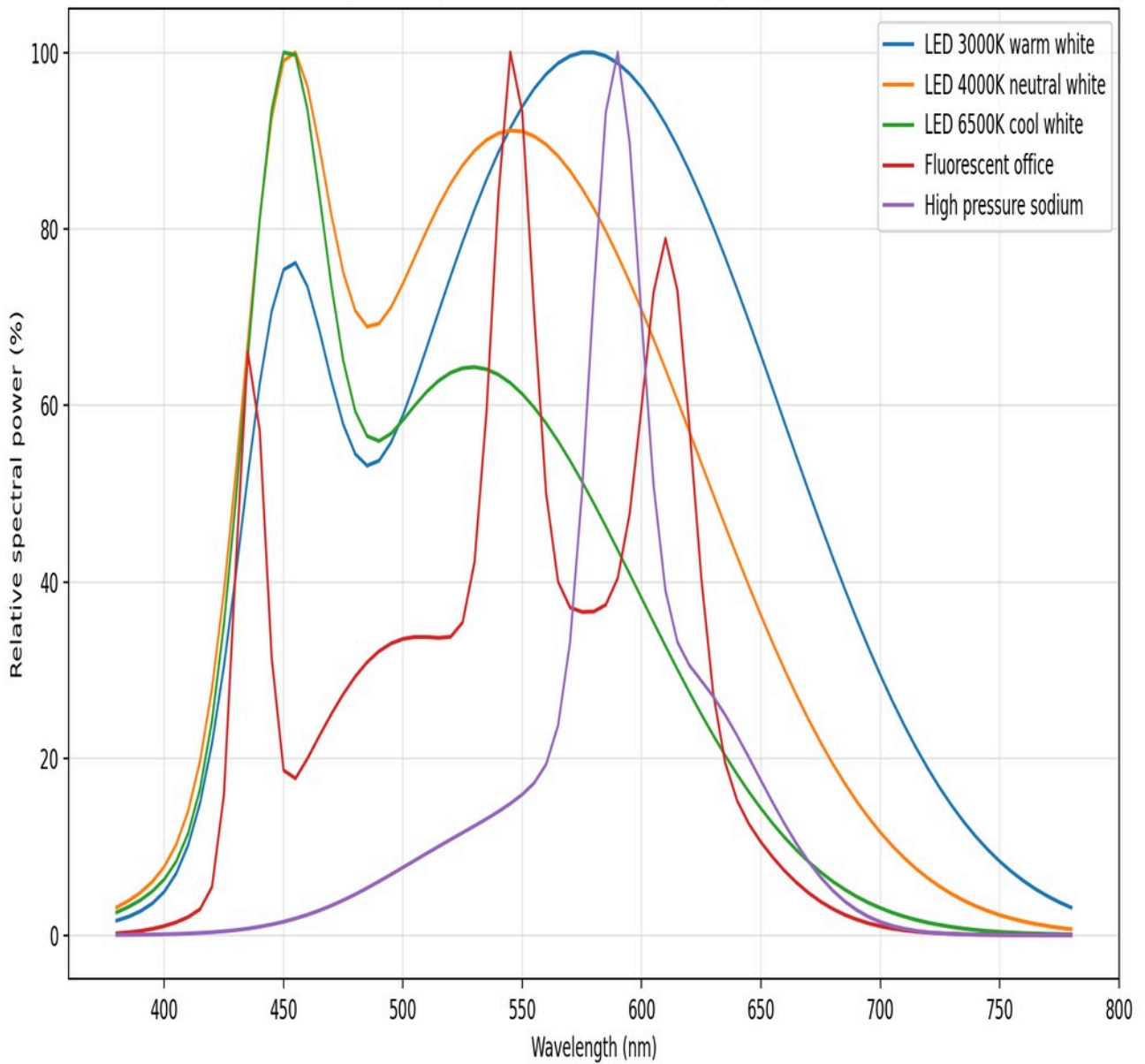
Synthetic Spectral Power Distribution for Lighting Fixtures
