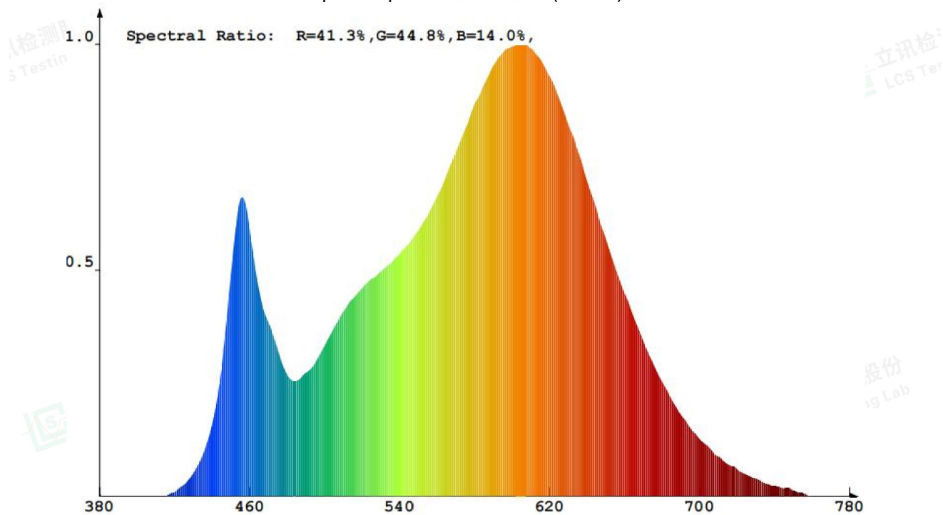
Spectral power distribution (3000K)
